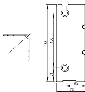
Corner fitting ON12 70x70x183
