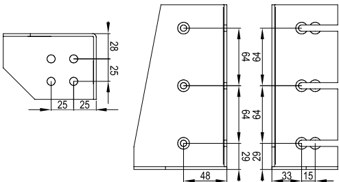
Corner fitting ON07 100x180x3
