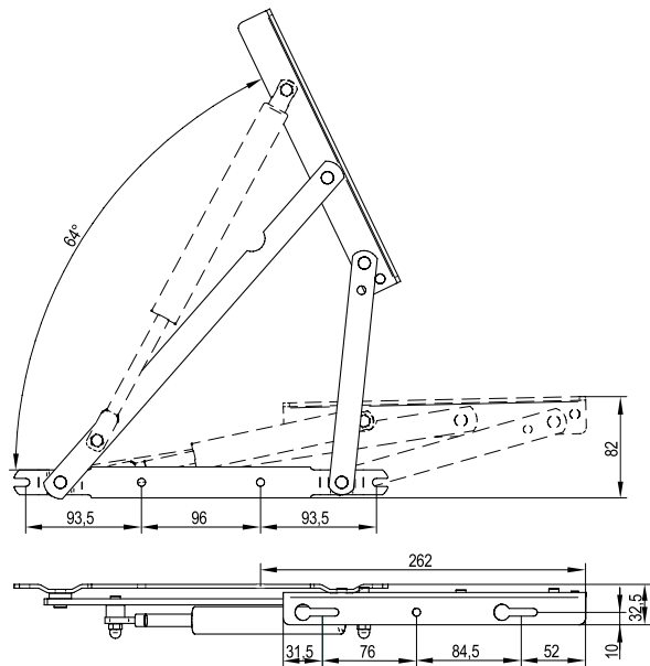
Bed frame lifter PR05
