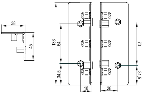
Corner fitting ON08 45x38x133
