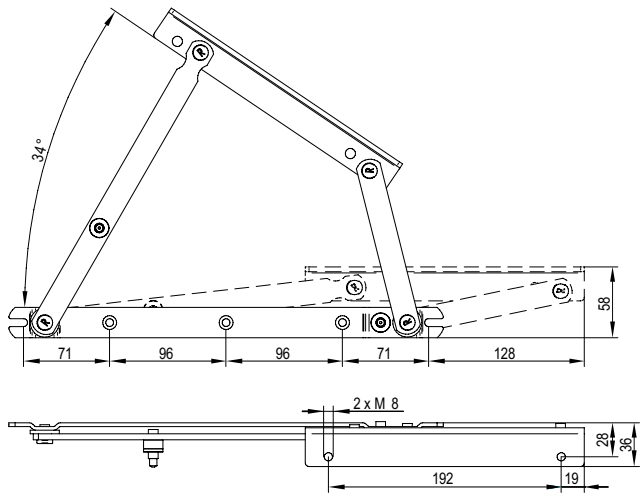
Bed frame lifter PR09
