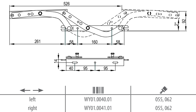
Tension spring 3x25x135 - F=200N
