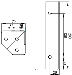
Corner fitting ON06 70x70x200
