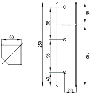
Corner fitting ON05 60x60x250
