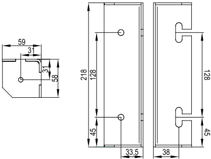
Corner fitting ON03 57x58x218
