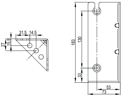
Corner fitting ON02 70x70x183
