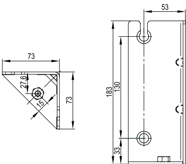
Corner fitting ON01 70x70x183
