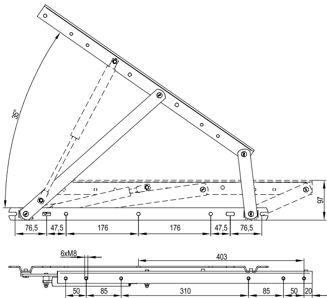
Bed frame lifter PR01
