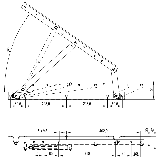
Bed frame lifter PR02
